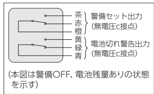
[EUCU-AD02内部回路]
